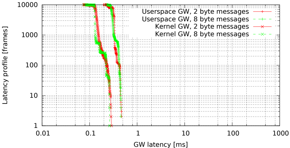
Kernel vs. userspace GW, no modifications (GW kernel 2.6.33.7-rt29-00004-g92487e4, Traffic oneatatime, Load none)
