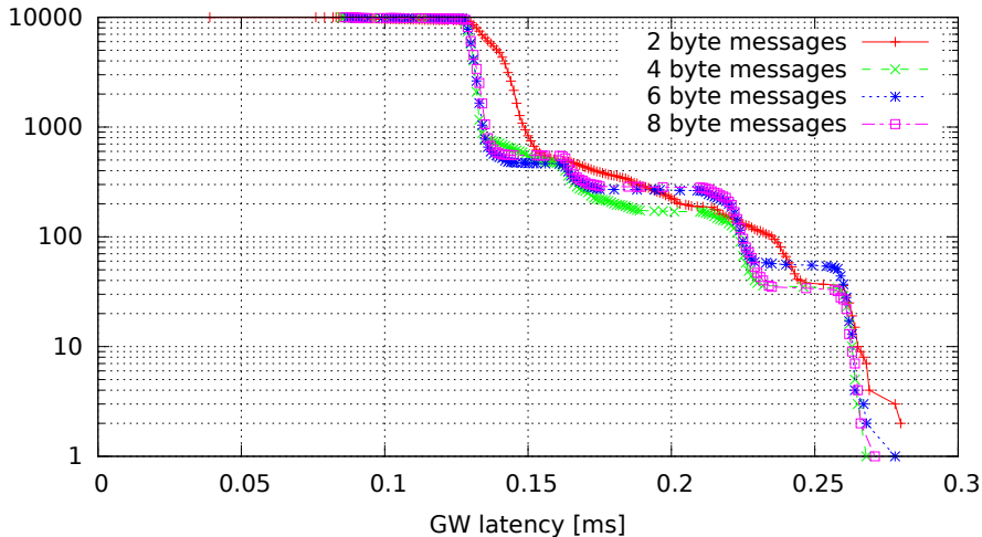
Single GW rule for all messages, no modifications (GW kernel 2.6.33.7-rt29-00004-g92487e4, Traffic oneatatime, Load none)
