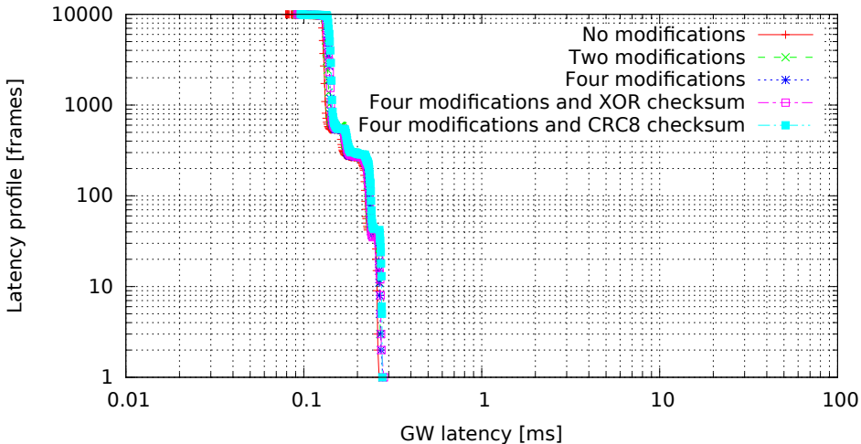
Single GW rule for all messages with modifications, 8 byte messages (GW kernel 2.6.33.7-rt29-00004-g92487e4, Traffic oneatatime, Load none)
