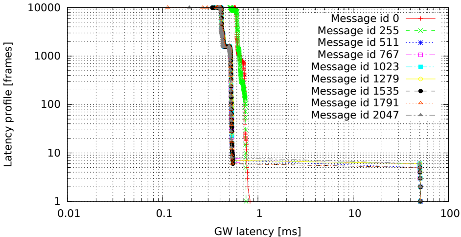
2048 GW rules (one per id, mask 0x7FF), no modifications (GW kernel 2.6.33.7-rt29-00004-g92487e4, Traffic oneatatime, Load none)
