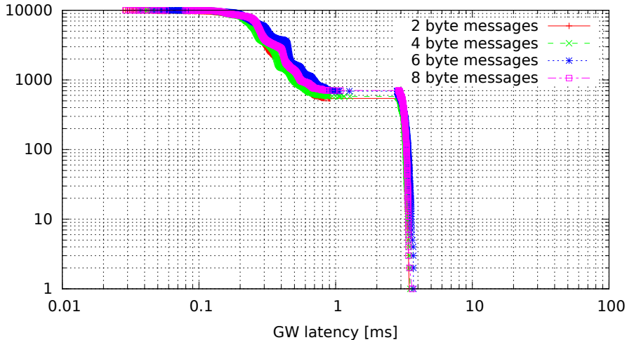
Single GW rule for all messages, no modifications (GW kernel 2.6.33.7-rt29-00004-g92487e4, Traffic oneatatime, Load eth)
