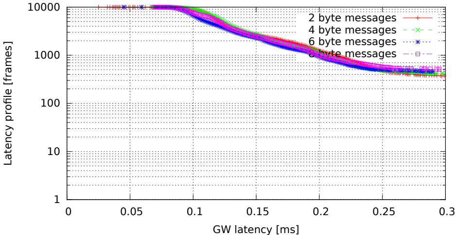
Single GW rule for all messages, no modifications, high (soft)irq task priority (GW kernel 2.6.33.7-rt29-00004-g92487e4, Traffic onetime, Load eth)
