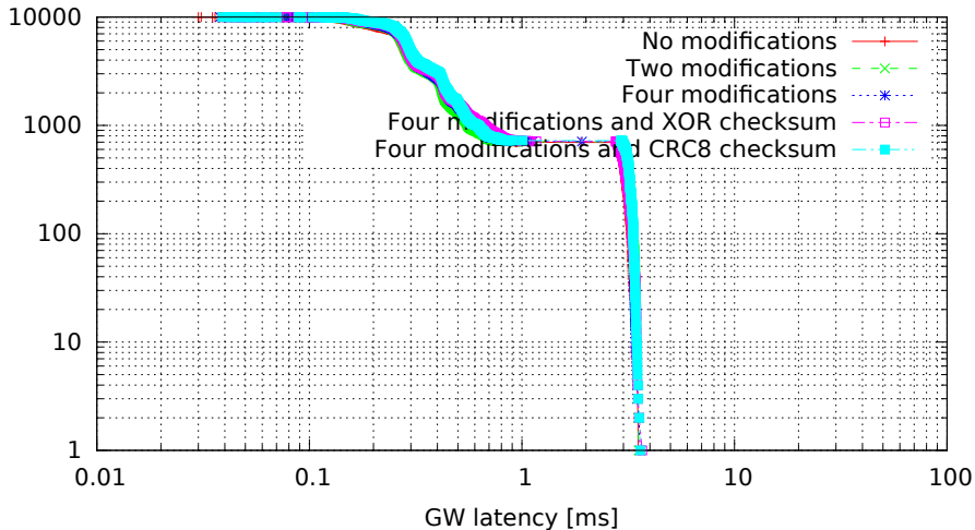
Single GW rule for all messages with modifications, 8 byte messages (GW kernel 2.6.33.7-rt29-00004-g92487e4, Traffic onetatime, Load eth)
