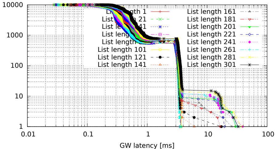
Different lengths of filter list, only the last one matches (GW kernel 2.6.33.7-rt29-00004-g92487e4, Traffic onetotime, Load eth)
