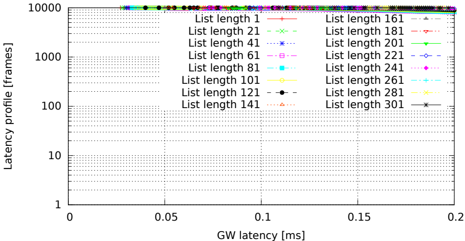
Different lengths of filter list, only the last one matches (GW kernel 2.6.33.7-rt29-00004-g92487e4, Traffic oneatatime, Load eth)
