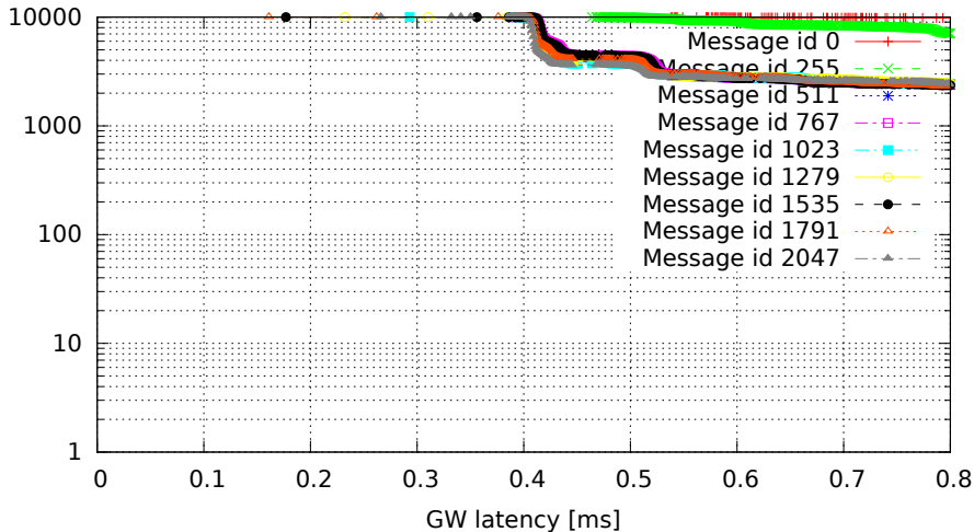
2048 GW rules (one per id, mask 0x7FF), no modifications (GW kernel 2.6.33.7-rt29-00004-g92487e4, Traffic onetime, Load eth)
