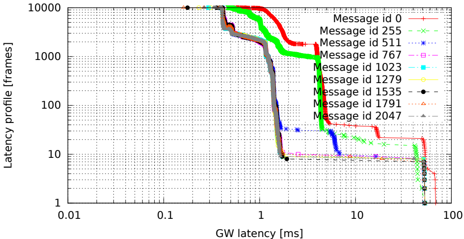
2048 GW rules (one per id, mask 0x7FF), no modifications (GW kernel 2.6.33.7-rt29-00004-g92487e4, Traffic onetatime, Load eth)
