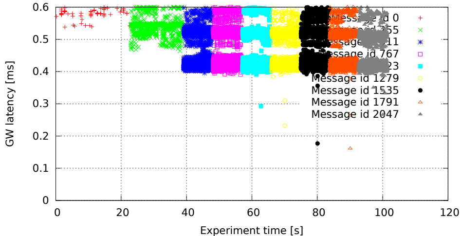
2048 GW rules (one per id, mask 0x7FF), no modifications (GW kernel 2.6.33.7-rt29-00004-g92487e4, Traffic oneatatime, Load eth)
