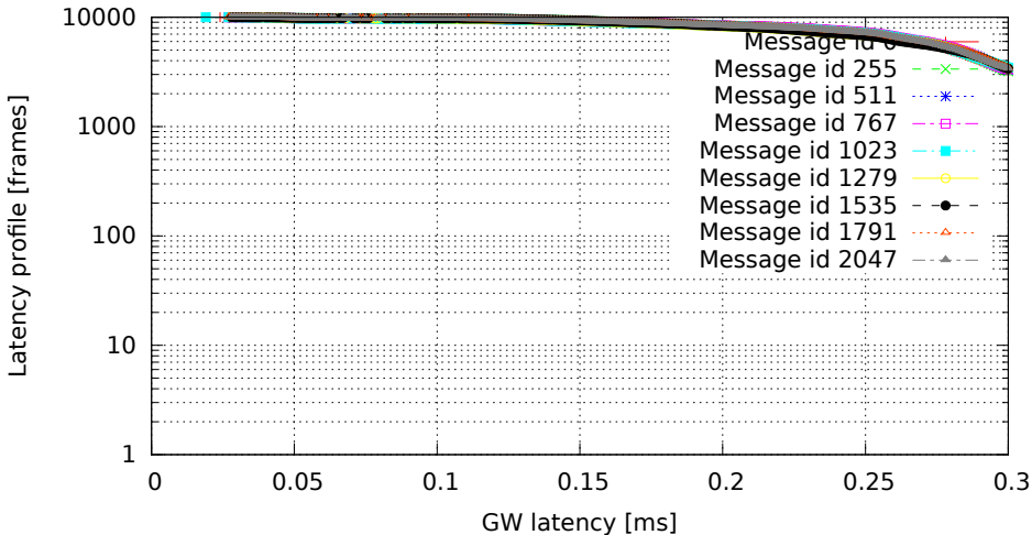
2048 GW rules (one per id, mask C00007FF), no modifications (GW kernel 2.6.33.7-rt29-00004-g92487e4, Traffic oneatatime, Load eth)
