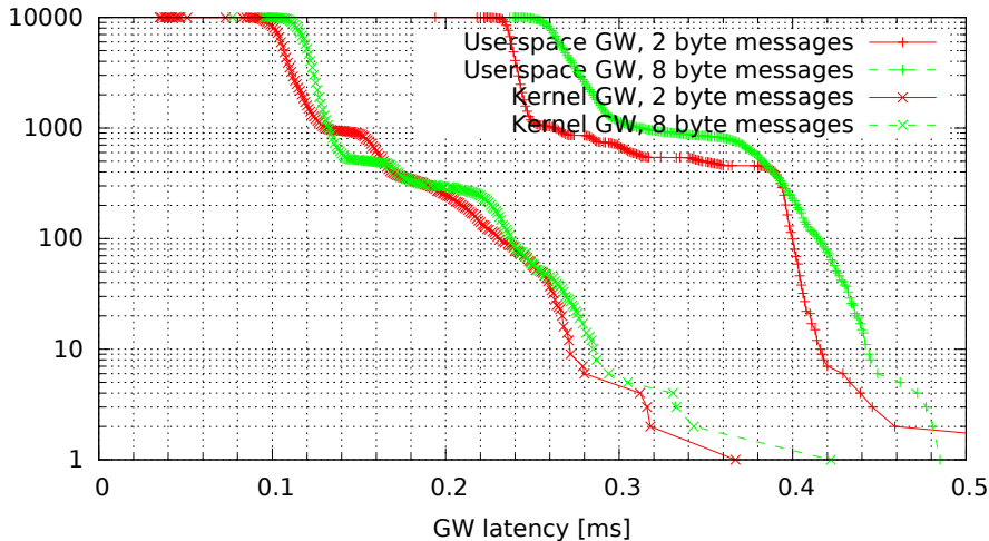
Kernel vs. userspace GW, no modifications (GW kernel 2.6.33.7-rt29-00004-g92487e4, Traffic oneatatime, Load cpu)
