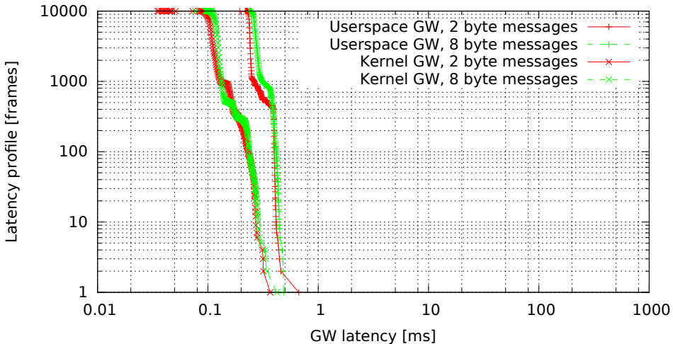
Kernel vs. userspace GW, no modifications (GW kernel 2.6.33.7-rt29-00004-g92487e4, Traffic oneatatime, Load cpu)
