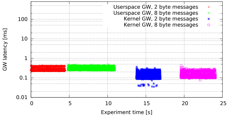
Single GW rule for all messages, no modifications (GW kernel 2.6.33.7-rt29-00004-g92487e4, Traffic oneatatime, Load cpu)
