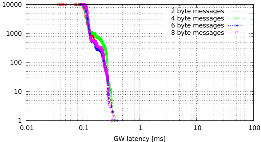
Single GW rule for all messages, no modifications (GW kernel 2.6.33.7-rt29-00004-g92487e4, Traffic oneatatime, Load cpu)
