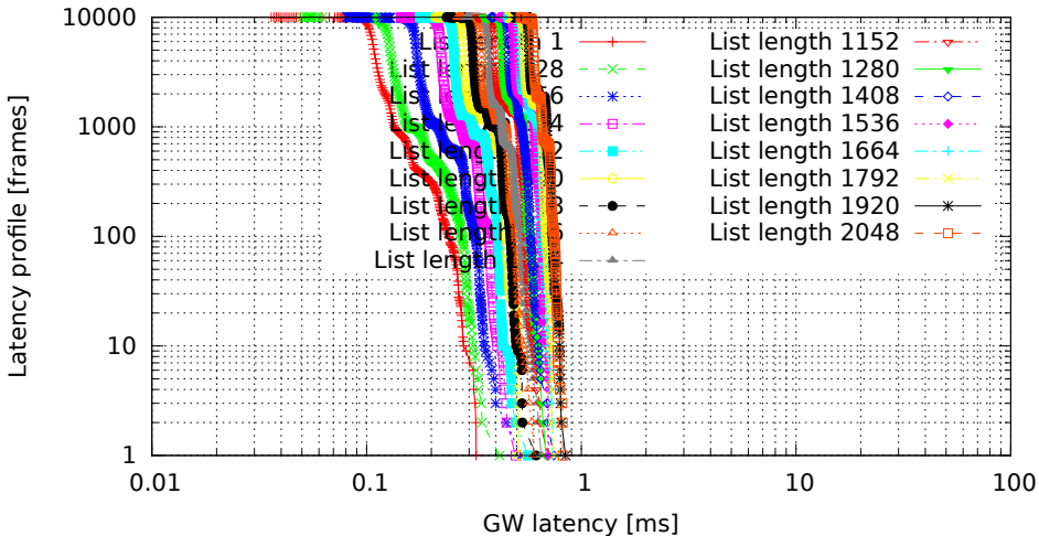
Different lengths of filter list, only the last one matches (GW kernel 2.6.33.7-rt29-00004-g92487e4, Traffic oneatatime, Load cpu)
