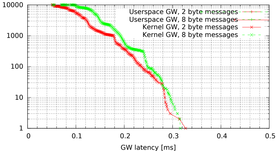
Kernel vs. userspace GW, no modifications (GW kernel 2.6.33.7-rt29-00004-g92487e4, Traffic flood, Load none)
