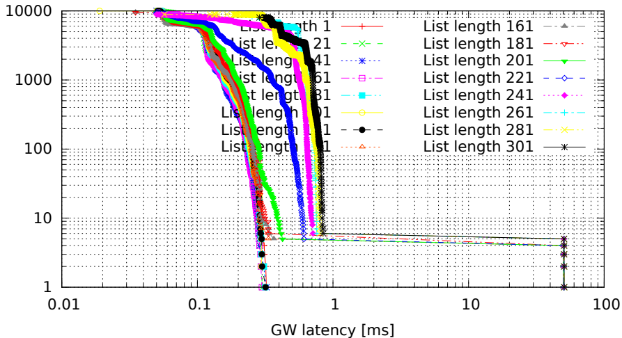
Different lengths of filter list, only the last one matches (GW kernel 2.6.33.7-rt29-00004-g92487e4, Traffic flood, Load none)
