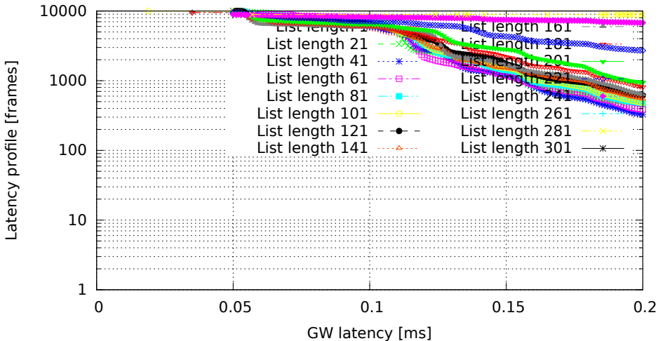
Different lengths of filter list, only the last one matches (GW kernel 2.6.33.7-rt29-00004-g92487e4, Traffic flood, Load none)
