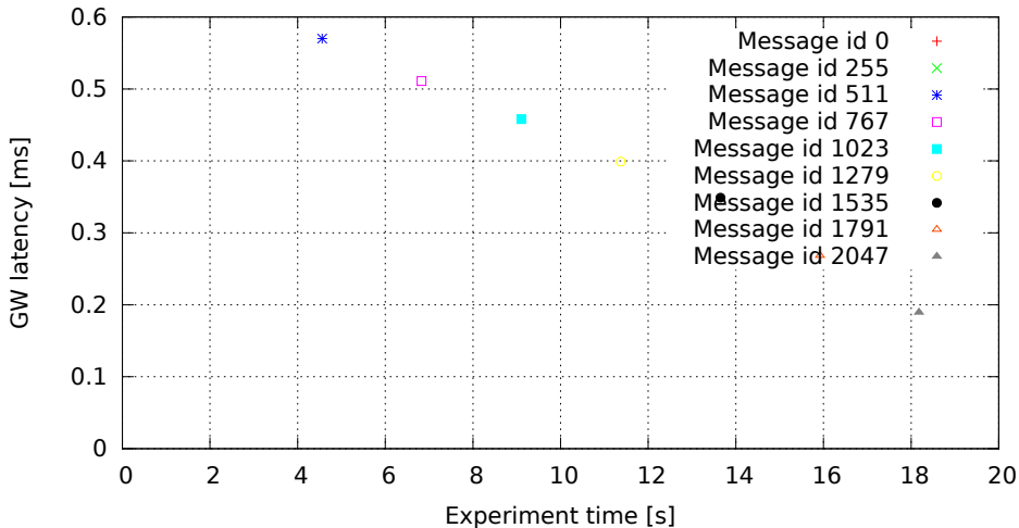
2048 GW rules (one per id, mask 0x7FF), no modifications (GW kernel 2.6.33.7-rt29-00004-g92487e4, Traffic flood, Load none)
