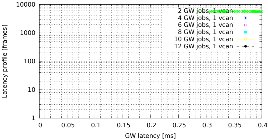
Chained GWs on a single VCAN interface (GW kernel 2.6.33.7-rt29-00004-g92487e4, Traffic flood, Load eth)
