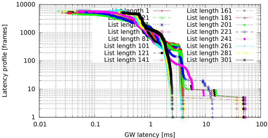
Different lengths of filter list, only the last one matches (GW kernel 2.6.33.7-rt29-00004-g92487e4, Traffic flood, Load eth)
