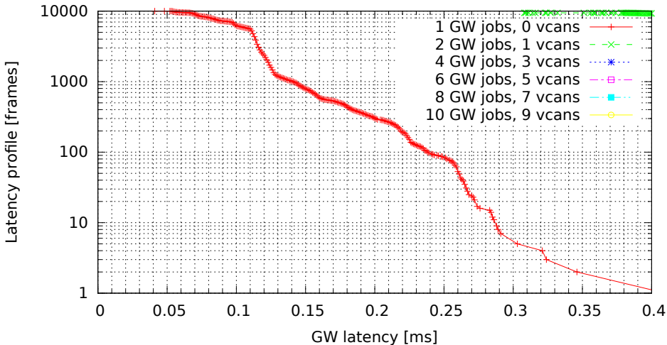
Chained GWs on multiple VCAN interfaces (GW kernel 2.6.33.7-rt29-00004-g92487e4, Traffic flood, Load cpu)
