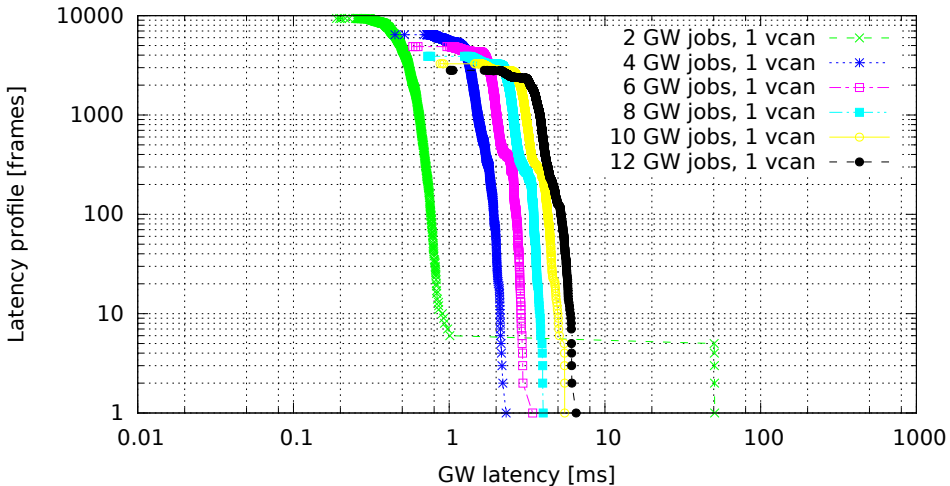
Chained GWs on a single VCAN interface (GW kernel 2.6.33.7-rt29-00004-g92487e4, Traffic flood, Load cpu)
