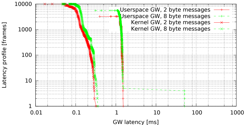
Kernel vs. userspace GW, no modifications (GW kernel 2.6.33.7-rt29-00004-g92487e4, Traffic flood, Load cpu)
