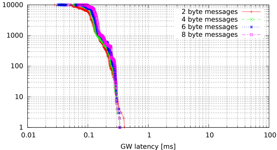
Single GW rule for all messages, no modifications (GW kernel 2.6.33.7-rt29-00004-g92487e4, Traffic flood, Load cpu)
