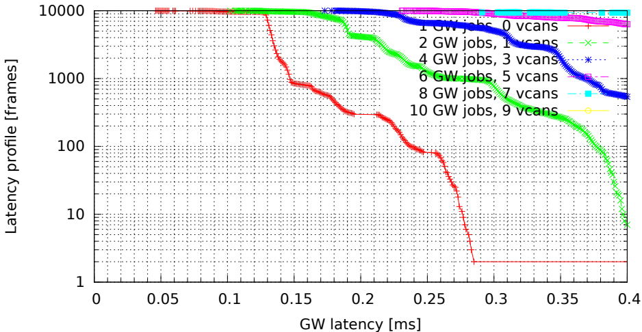
Chained GWs on multiple VCAN interfaces (GW kernel 2.6.33.7-rt29-00004-g92487e4, Traffic 50, Load none)
