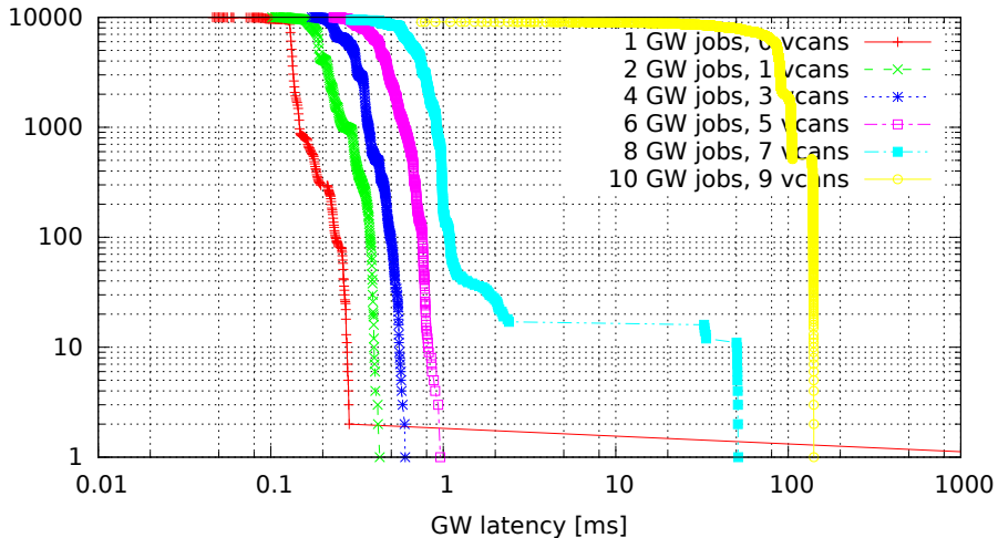
Chained GWs on multiple VCAN interfaces (GW kernel 2.6.33.7-rt29-00004-g92487e4, Traffic 50, Load none)
