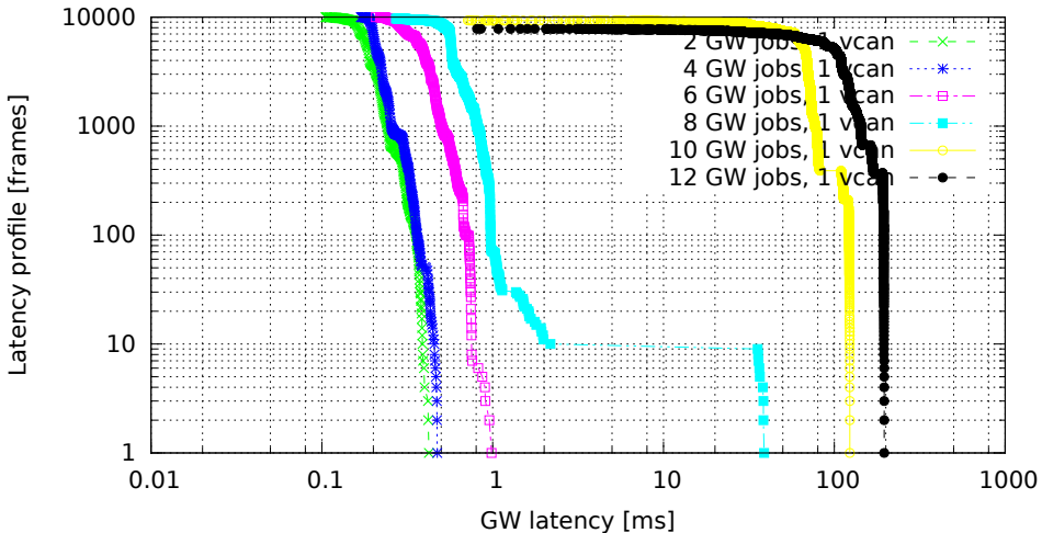
Chained GWs on a single VCAN interface (GW kernel 2.6.33.7-rt29-00004-g92487e4, Traffic 50, Load none)
