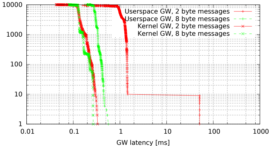
Kernel vs. userspace GW, no modifications (GW kernel 2.6.33.7-rt29-00004-g92487e4, Traffic 50, Load none)
