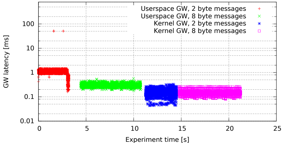
Single GW rule for all messages, no modifications (GW kernel 2.6.33.7-rt29-00004-g92487e4, Traffic 50, Load none)
