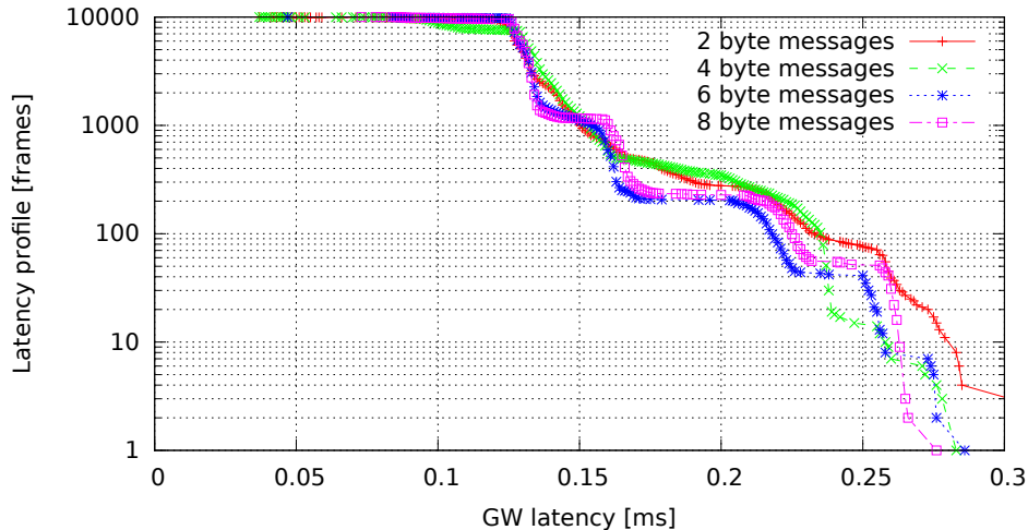
Single GW rule for all messages, no modifications (GW kernel 2.6.33.7-rt29-00004-g92487e4, Traffic 50, Load none)
