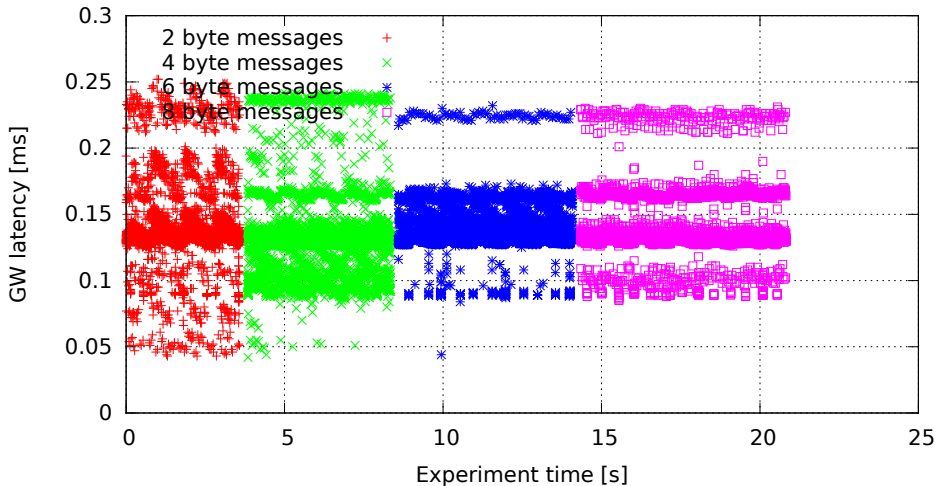
Single GW rule for all messages, no modifications, high (soft)irq task priority (GW kernel 2.6.33.7-rt29-00004-g92487e4, Traffic 50, Load none)
