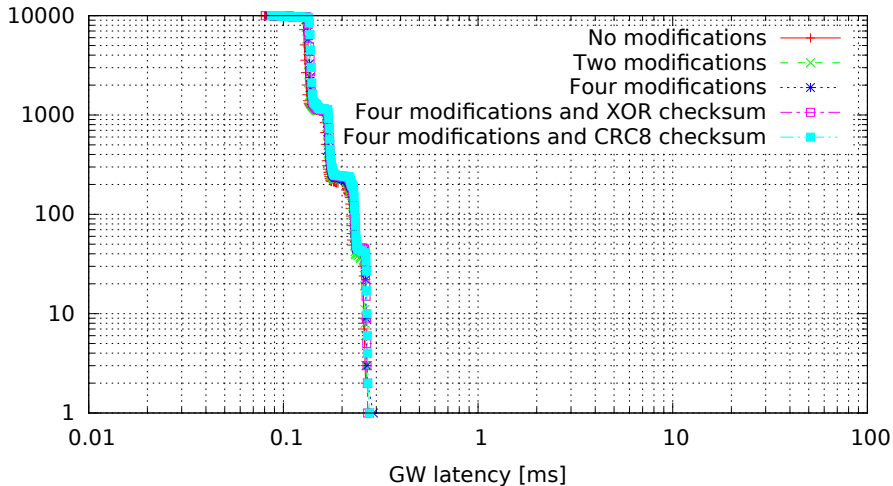
Single GW rule for all messages with modifications, 8 byte messages (GW kernel 2.6.33.7-rt29-00004-g92487e4, Traffic 50, Load none)
