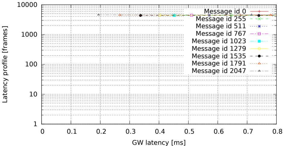
2048 GW rules (one per id, mask 0x7FF), no modifications (GW kernel 2.6.33.7-rt29-00004-g92487e4, Traffic 50, Load none)
