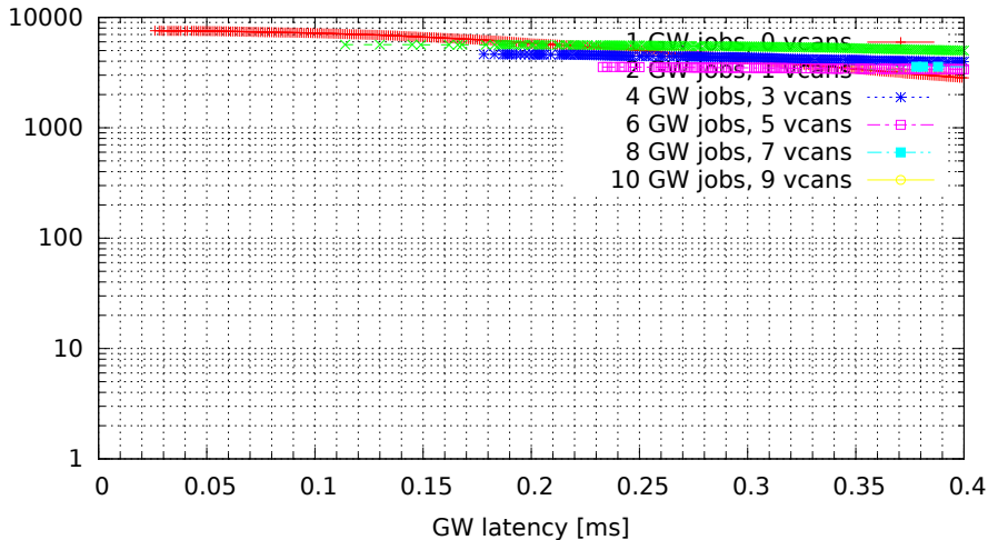
Chained GWs on multiple VCAN interfaces (GW kernel 2.6.33.7-rt29-00004-g92487e4, Traffic 50, Load eth)
