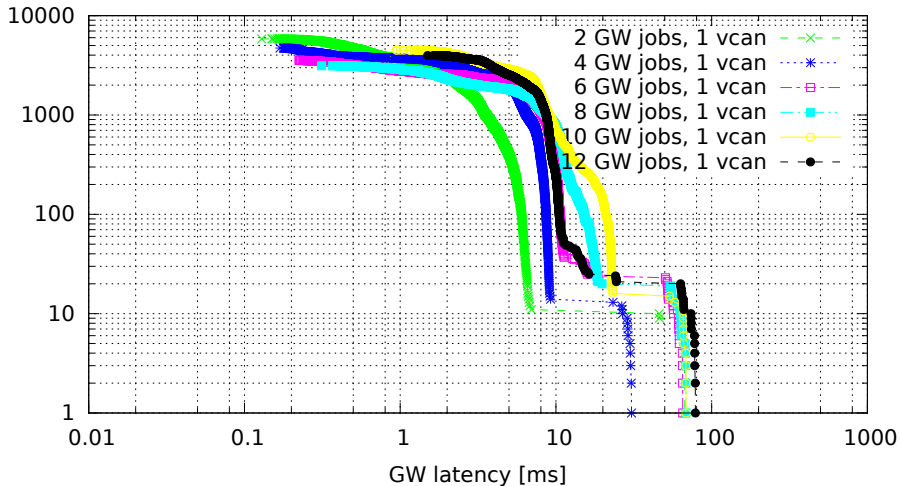
Chained GWs on a single VCAN interface (GW kernel 2.6.33.7-rt29-00004-g92487e4, Traffic 50, Load eth)
