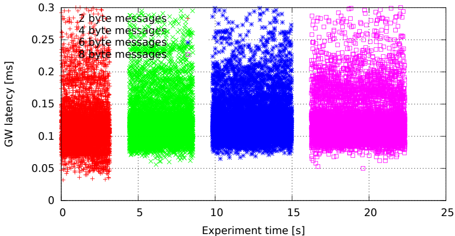
Single GW rule for all messages, no modifications, high (soft)irq task priority (GW kernel 2.6.33.7-rt29-00004-g92487e4, Traffic 50, Load eth)
