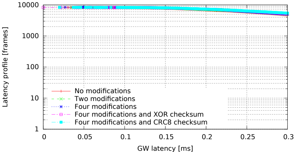
Single GW rule for all messages with modifications, 8 byte messages (GW kernel 2.6.33.7-rt29-00004-g92487e4, Traffic 50, Load eth)
