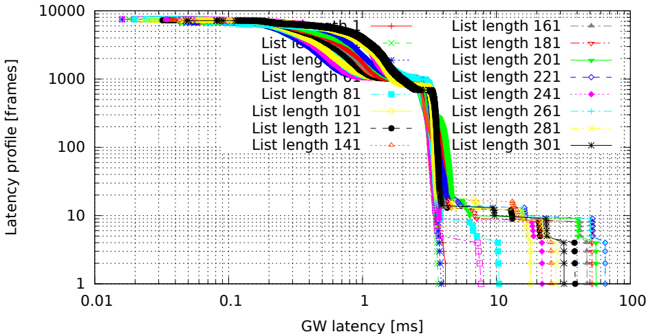
Different lengths of filter list, only the last one matches (GW kernel 2.6.33.7-rt29-00004-g92487e4, Traffic 50, Load eth)
