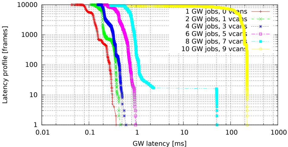
Chained GWs on multiple VCAN interfaces (GW kernel 2.6.33.7-rt29-00004-g92487e4, Traffic 50, Load cpu)
