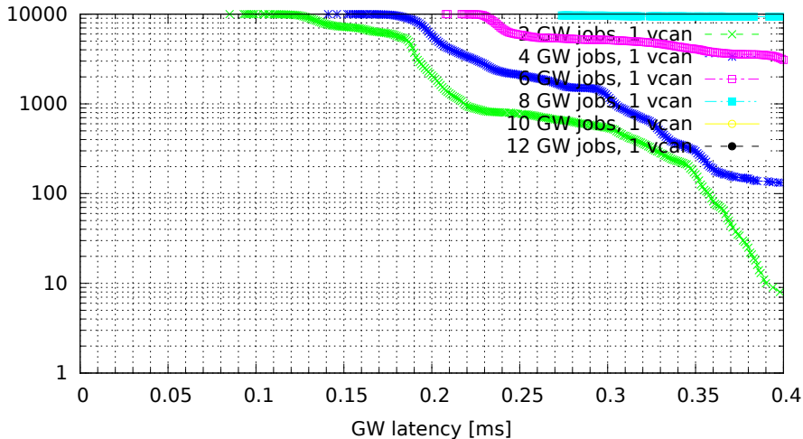
Chained GWs on a single VCAN interface (GW kernel 2.6.33.7-rt29-00004-g92487e4, Traffic 50, Load cpu)
