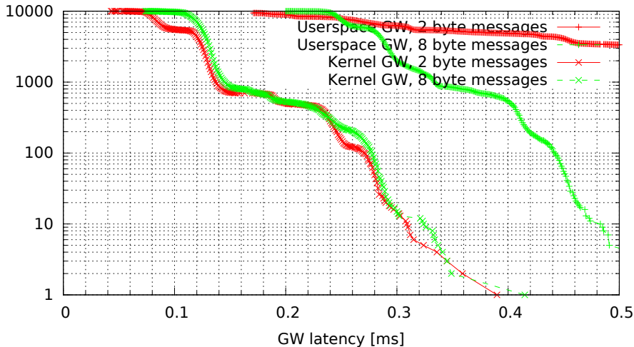
Kernel vs. userspace GW, no modifications (GW kernel 2.6.33.7-rt29-00004-g92487e4, Traffic 50, Load cpu)
