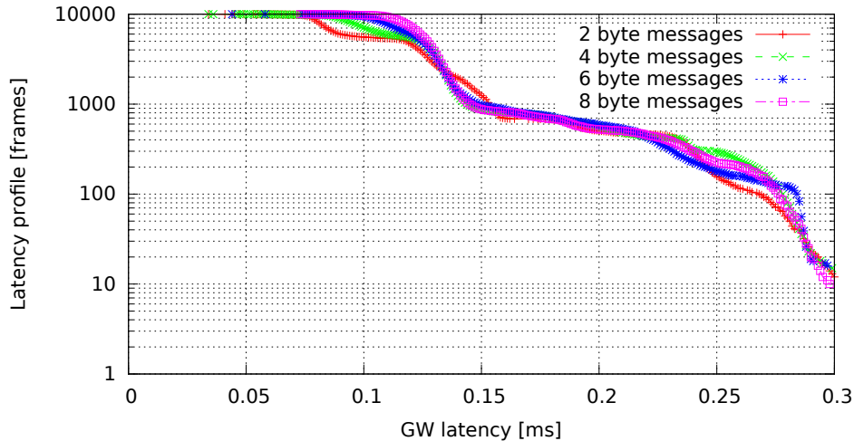
Single GW rule for all messages, no modifications (GW kernel 2.6.33.7-rt29-00004-g92487e4, Traffic 50, Load cpu)
