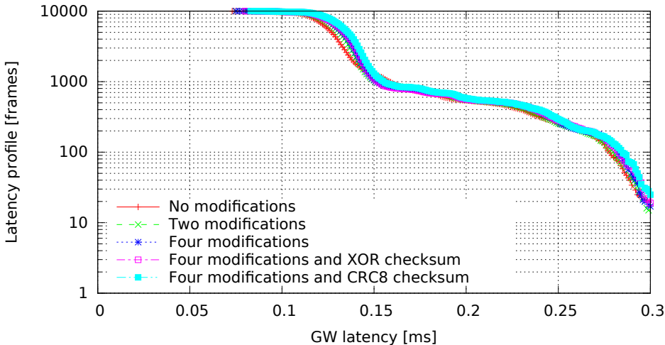
Single GW rule for all messages with modifications, 8 byte messages (GW kernel 2.6.33.7-rt29-00004-g92487e4, Traffic 50, Load cpu)
