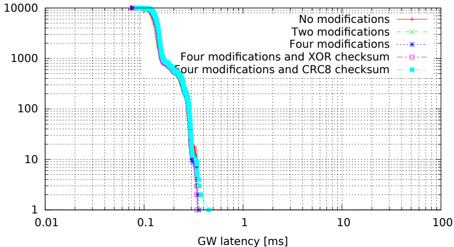
Single GW rule for all messages with modifications, 8 byte messages (GW kernel 2.6.33.7-rt29-00004-g92487e4, Traffic 50, Load cpu)
