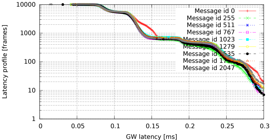
2048 GW rules (one per id, mask C00007FF), no modifications (GW kernel 2.6.33.7-rt29-00004-g92487e4, Traffic 50, Load cpu)
