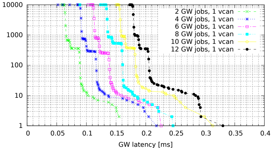
Chained GWs on a single VCAN interface (GW kernel 2.6.33.7-00007-g9c0ff90, Traffic oneatatime, Load none)
